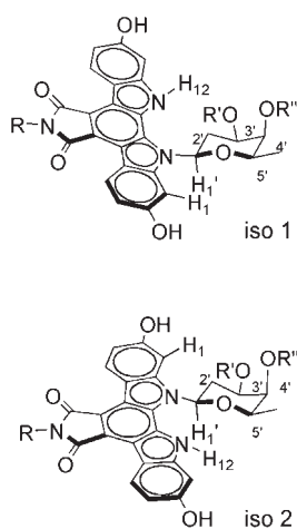
Figure 6. Structures of the two conformations iso1 and iso2 for compounds 1 [ R = \text{NH}(\text{CH}_2\text{OH})_2 ; R' = \text{H} ; R'' = 2\text{-deoxy-}\alpha\text{-L-fucose} ] and 2 [ R = \text{NH}(\text{CH}_2\text{OH})_2 ; R' = 2\text{-deoxy-}\alpha\text{-L-fucose} ; R'' = \text{H} ].
