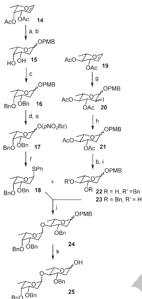
Scheme 1. Reagents and conditions: a) p -MeOBnOH (2 equiv), (Ph) 3 PHBr (0.05 equiv), CH 2 Cl 2 , 20 °C, 3 h, 60%; b) MeONa (0.3 equiv), MeOH, 0 → 20 °C, 1 h, quant.; c) BnCl (5 equiv), KOH, dioxane, reflux, 88%; d) Ce(NH 4 ) 2 (NO 3 ) 6 (2 equiv), CH 3 CN/H 2 O (9:1), 20 °C, 3 h, 90%; e) p -NO 2 BzCl (3 equiv), DMAP (0.1 equiv), pyridine (3 equiv), CH 2 Cl 2 , 20 °C, 82%; f) PhSSi(Me) 3 (4.5 equiv), CF 3 SO 3 Si(Me) 3 (2.5 equiv), CH 2 Cl 2 , 0 → 20 °C, 24 h, 88%; g) p -MeOBnOH (2 equiv), NIS (1.6 equiv), CH 3 CN, 20 °C, 24 h, 90%; h) Bu 3 SnH (1.4 equiv), AIBN (0.15 equiv), toluene, 80 °C, 4 h, 90%; i) BnCl (2 equiv), KOH, dioxane, 20 °C, 65%; j) IDCP (2 equiv), molecular sieves 4 Å, Et 2 O/1,2-dichloroethane (4:1), 20 °C, 4 h, 90%; k) DDQ (1.4 equiv), CH 2 Cl 2 /H 2 O (50:1), 20 °C, 30 min, 50%. AIBN = azobisisobutyronitrile, IDCP = iodonium dicollidine perchlorate, NIS = N -iodosuccinimide, PMB = para -methoxybenzyl.
